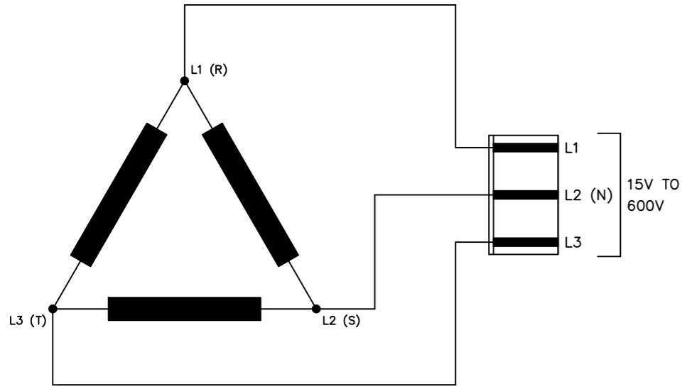
3 PHASE, 3 WIRE DELTA
