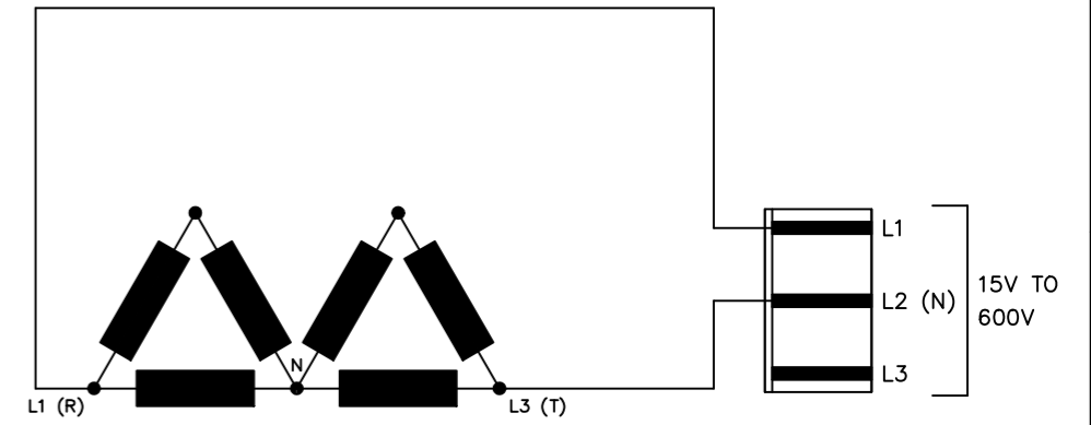
2 PHASE (L1 & L3), 3 WIRE DELTA / SINGLE PHASE, 3 WIRE
