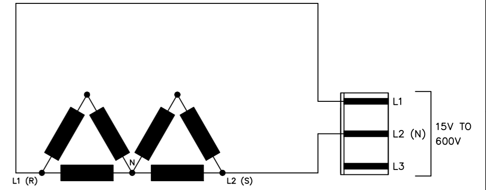
2 PHASE (L1 & L2), 3 WIRE DELTA / SINGLE PHASE, 3 WIRE
