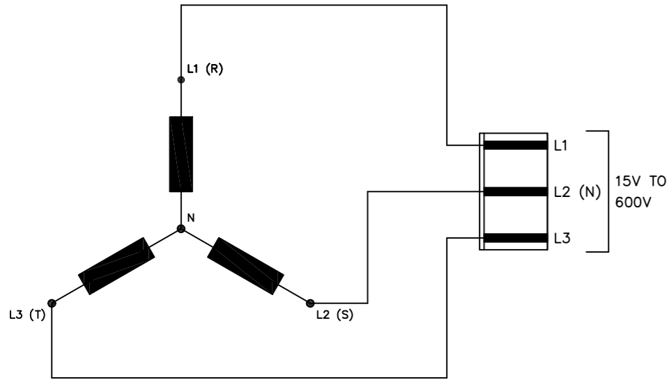
3 PHASE, 4 WIRE STAR
