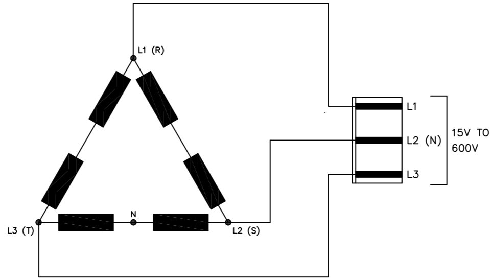
3 PHASE, 4 WIRE DELTA
