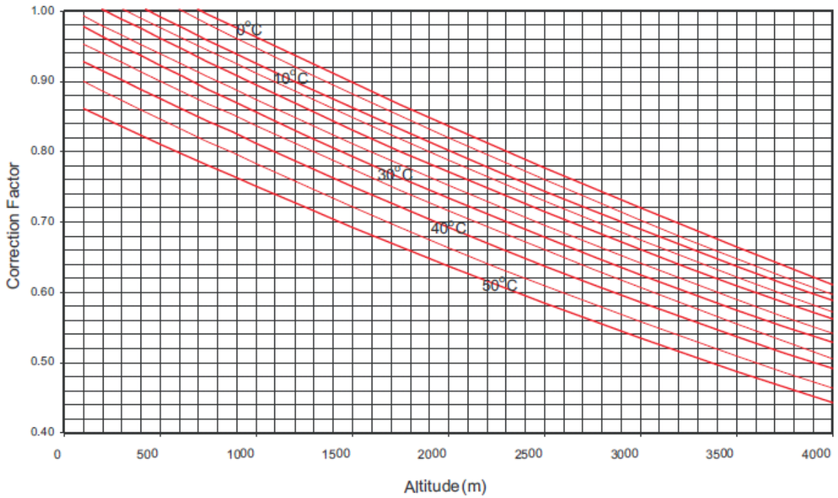
CHART A: Naturally aspirated Gen Motor engines stationary - BFM3
