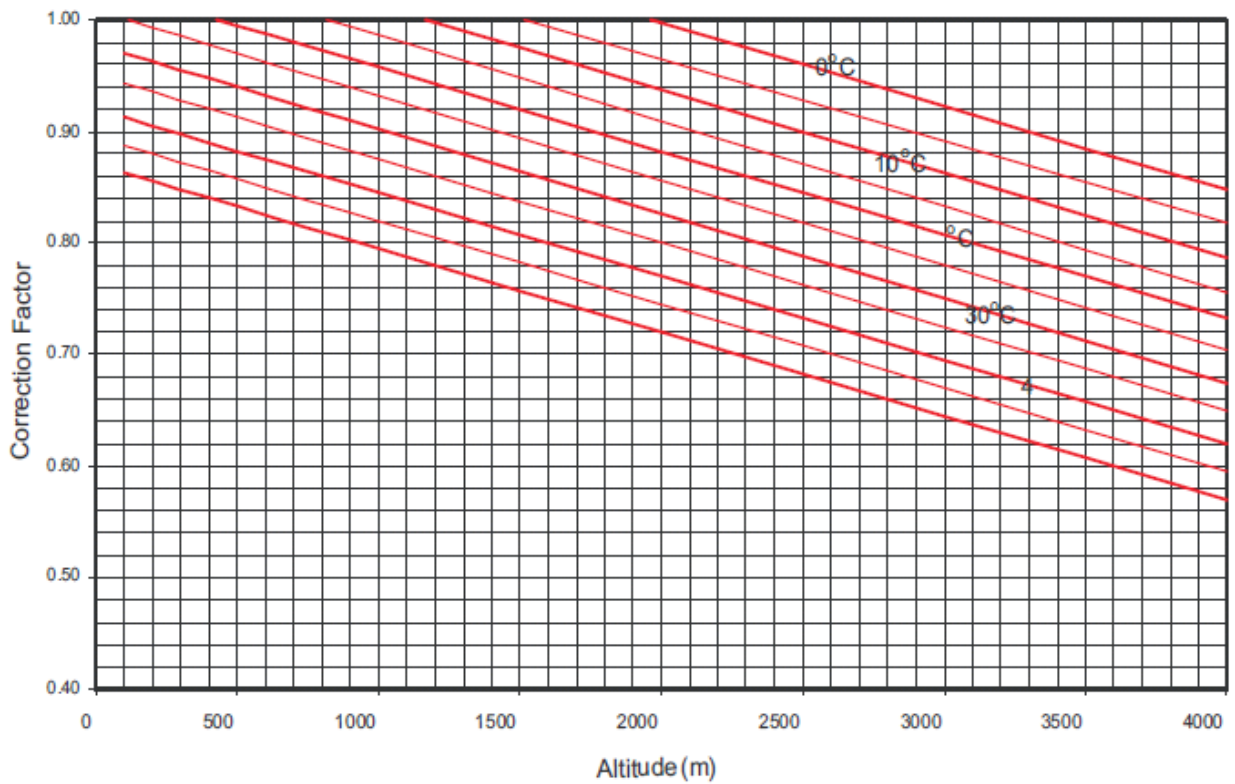
CHART B: Turbo-charged Gen Motor engines stationary - BFM3T/C
